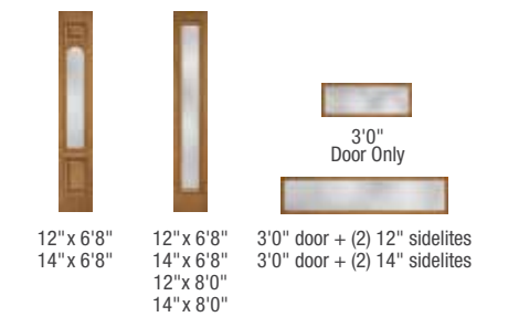
3'0" x 8'0" 3'0" x 8'0" 12" x 6'8" 14" x 6'8" 12" x 6'8" 14" x 6'8" 14" x 6'8"
